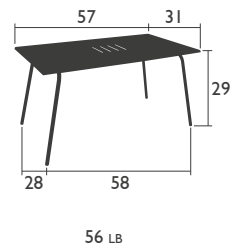
4831 - TABLE 57 X 31 INCH Tubular steel frame Electrogalvanized sheet steel table top with "slat effect" laser cutting
