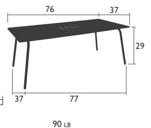
4832 - TABLE 76 X 37 INCH Tubular steel frame Electrogalvanized sheet steel table top with "slat effect" laser cutting
